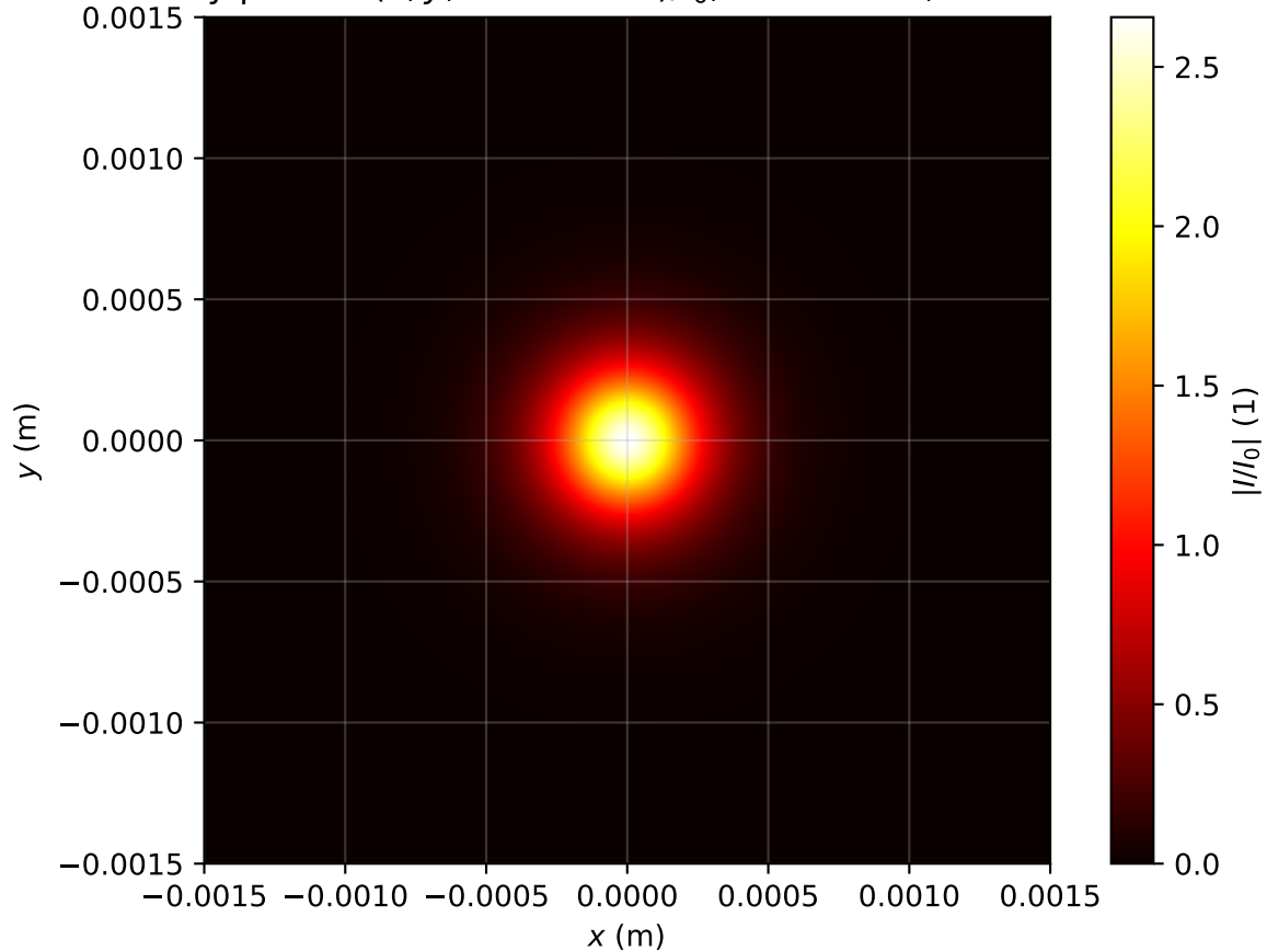
Intensity profile I(x, y, z = 3.025m)/I_0 , Pin=1.0Pcr, artificial time
